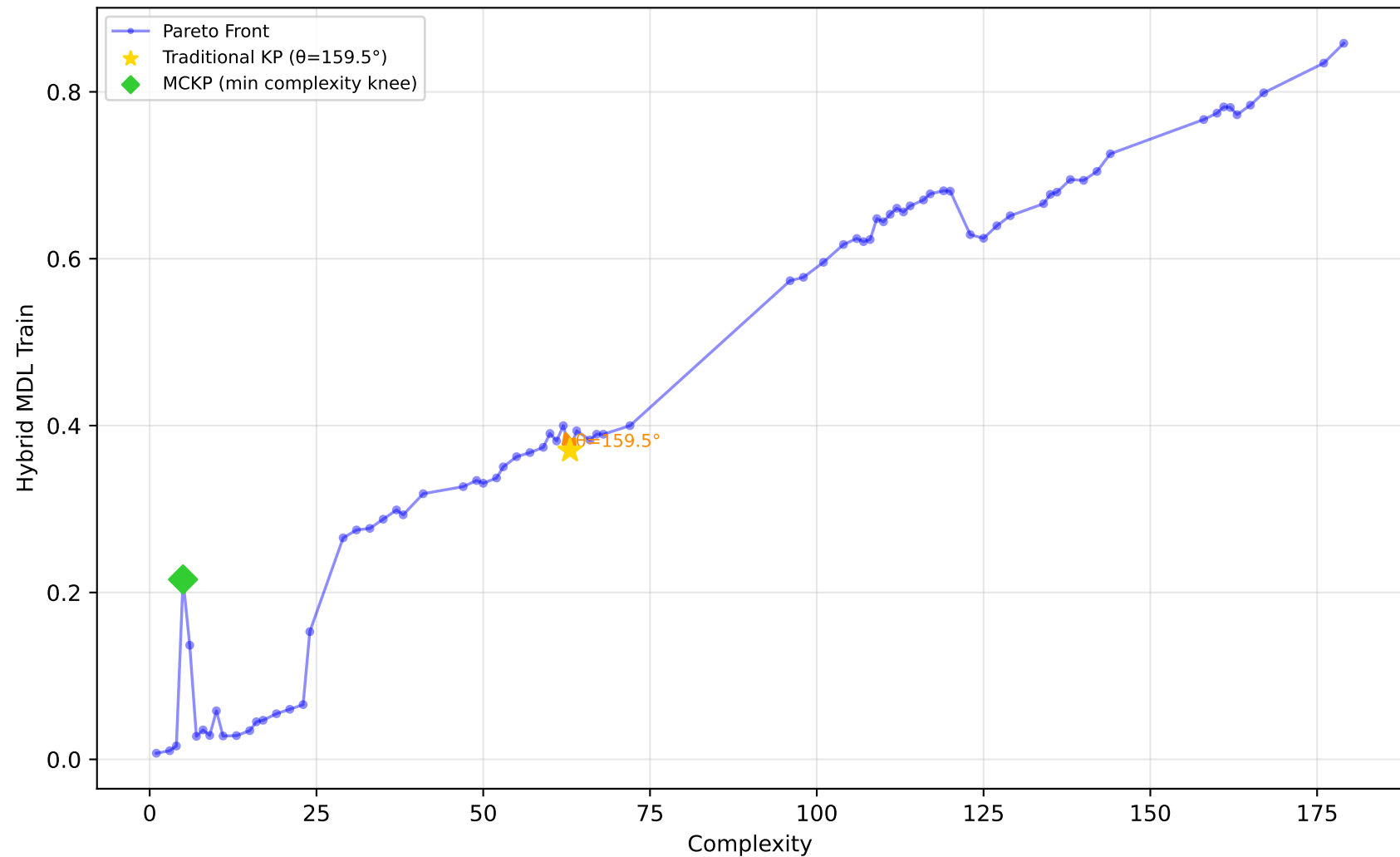
542_pollution - Run 29 - SVP - Hybrid MDL Train \lambda_1=0.00, \lambda_2=0.00, \lambda_3=0.20 | Difficulty: 1.00 | Method: hmr
