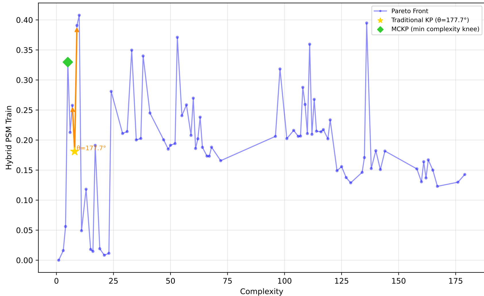
542_pollution - Run 29 - SVP - Hybrid PSM Train \lambda_1=0.00 , \bar{\lambda}_2=0.00 , \lambda_3=0.20 | Difficulty: 1.00 | Method: hmr
