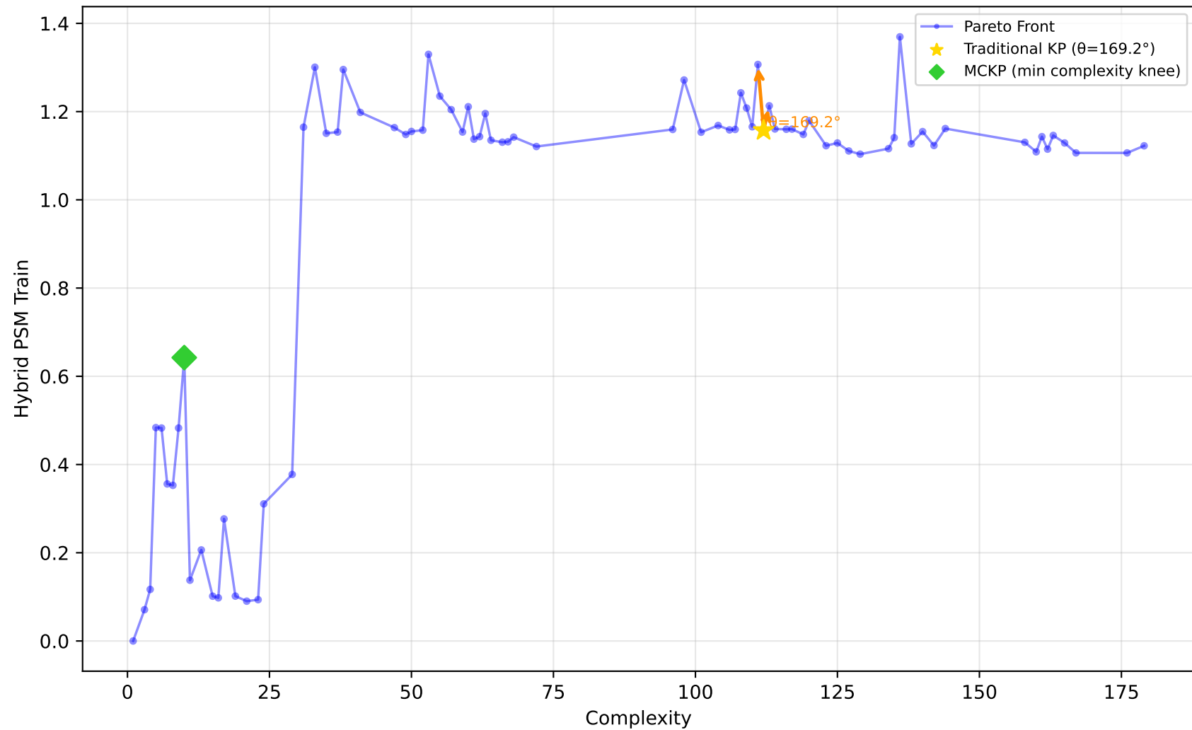
542_pollution - Run 29 - SVP - Hybrid PSM Train \lambda_1=0.70 , \lambda_2=1.00 , \lambda_3=0.10 | Difficulty: 1.00 | Method: hmr
