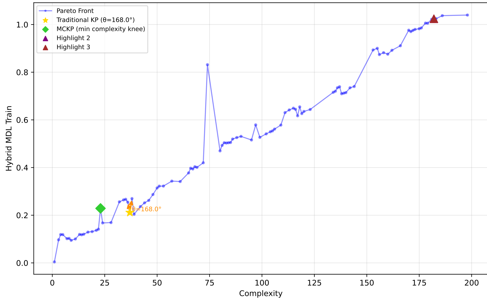
542_pollution - Run 2 - MVP - Hybrid MDL Train \lambda_1=1.00, \lambda_2=0.10, \lambda_3=0.00 | Difficulty: 0.51 | Method: mckp
