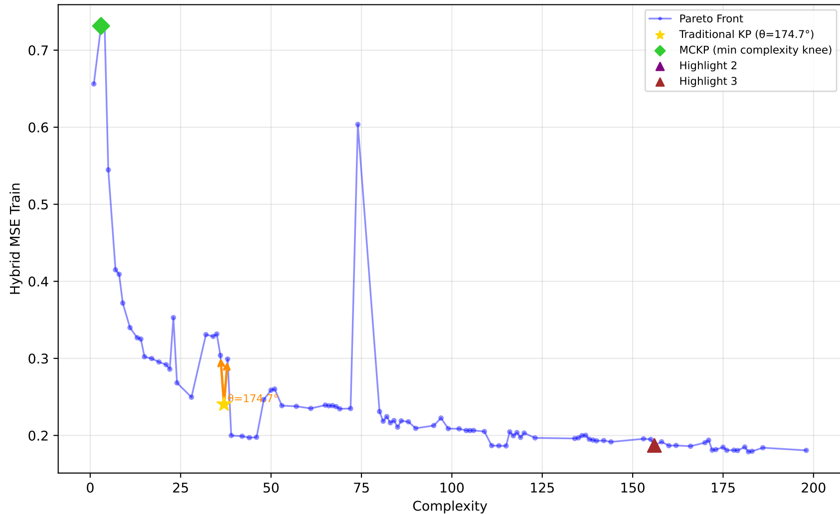
542_pollution - Run 2 - MVP - Hybrid MSE Train \lambda_1=1.00, \lambda_2=0.10, \lambda_3=0.00 | Difficulty: 0.51 | Method: mckp
