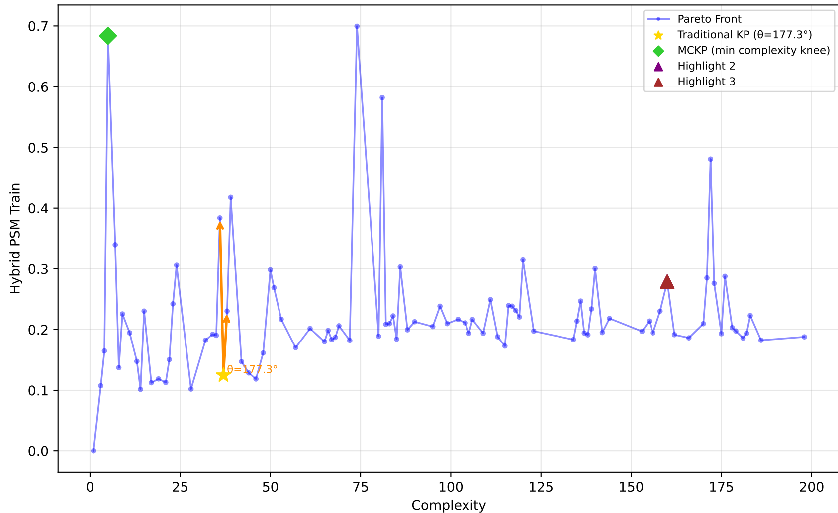
542_pollution - Run 2 - MVP - Hybrid PSM Train \lambda_1=1.00, \lambda_2=0.10, \lambda_3=0.00 | Difficulty: 0.51 | Method: mckp
