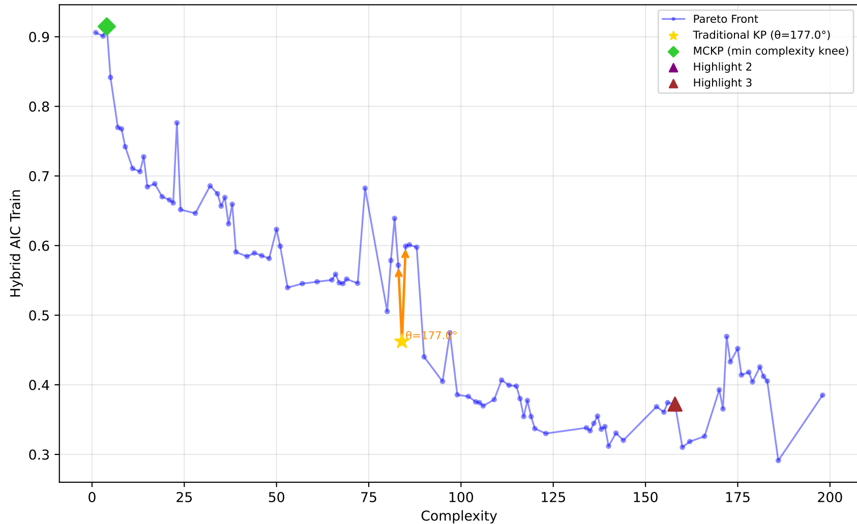
542_pollution - Run 2 - SVP - Hybrid AIC Train \lambda_1=0.00, \lambda_2=0.00, \lambda_3=0.20 | Difficulty: 0.51 | Method: mckp
