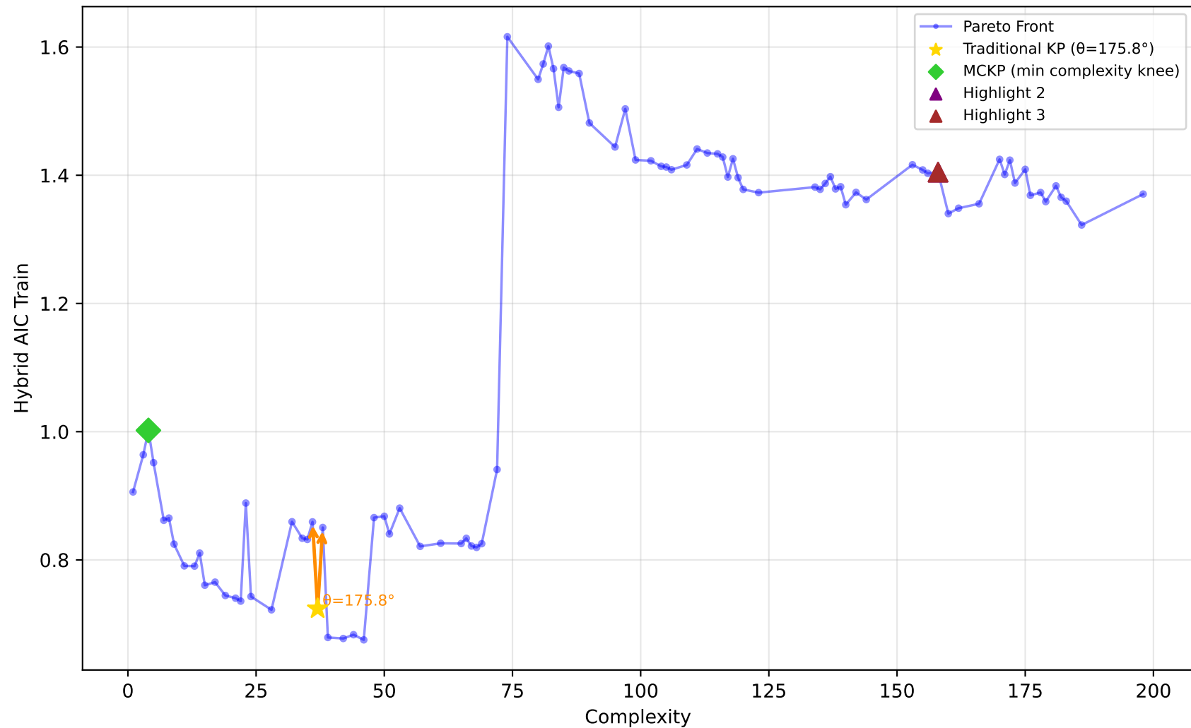
542_pollution - Run 2 - SVP - Hybrid AIC Train \lambda_1=0.70, \lambda_2=1.00, \lambda_3=0.10 | Difficulty: 0.51 | Method: mckp
