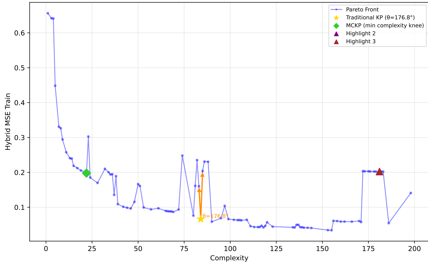
542_pollution - Run 2 - SVP - Hybrid MSE Train \lambda_1=0.00, \lambda_2=0.00, \lambda_3=0.20 | Difficulty: 0.51 | Method: mckp
