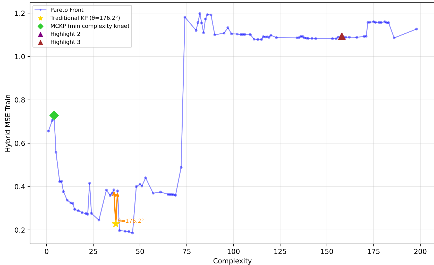
542_pollution - Run 2 - SVP - Hybrid MSE Train \lambda_1=0.70, \lambda_2=1.00, \lambda_3=0.10 | Difficulty: 0.51 | Method: mckp
