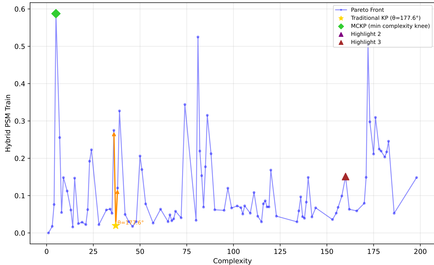
542_pollution - Run 2 - SVP - Hybrid PSM Train \lambda_1=0.00, \lambda_2=0.00, \lambda_3=0.20 | Difficulty: 0.51 | Method: mckp
