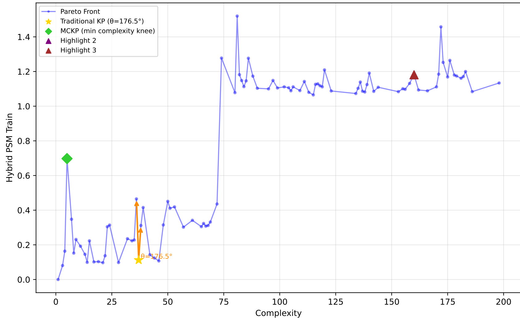
542_pollution - Run 2 - SVP - Hybrid PSM Train \lambda_1=0.70 , \lambda_2=1.00 , \lambda_3=0.10 | Difficulty: 0.51 | Method: mckp
