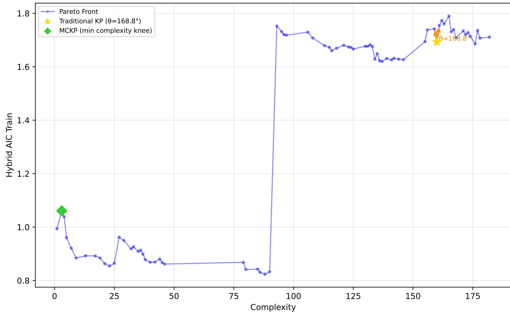
542_pollution - Run 30 - MVP - Hybrid AIC Train \lambda_1=1.00, \lambda_2=0.10, \lambda_3=0.00 | Difficulty: 0.24 | Method: mckp
