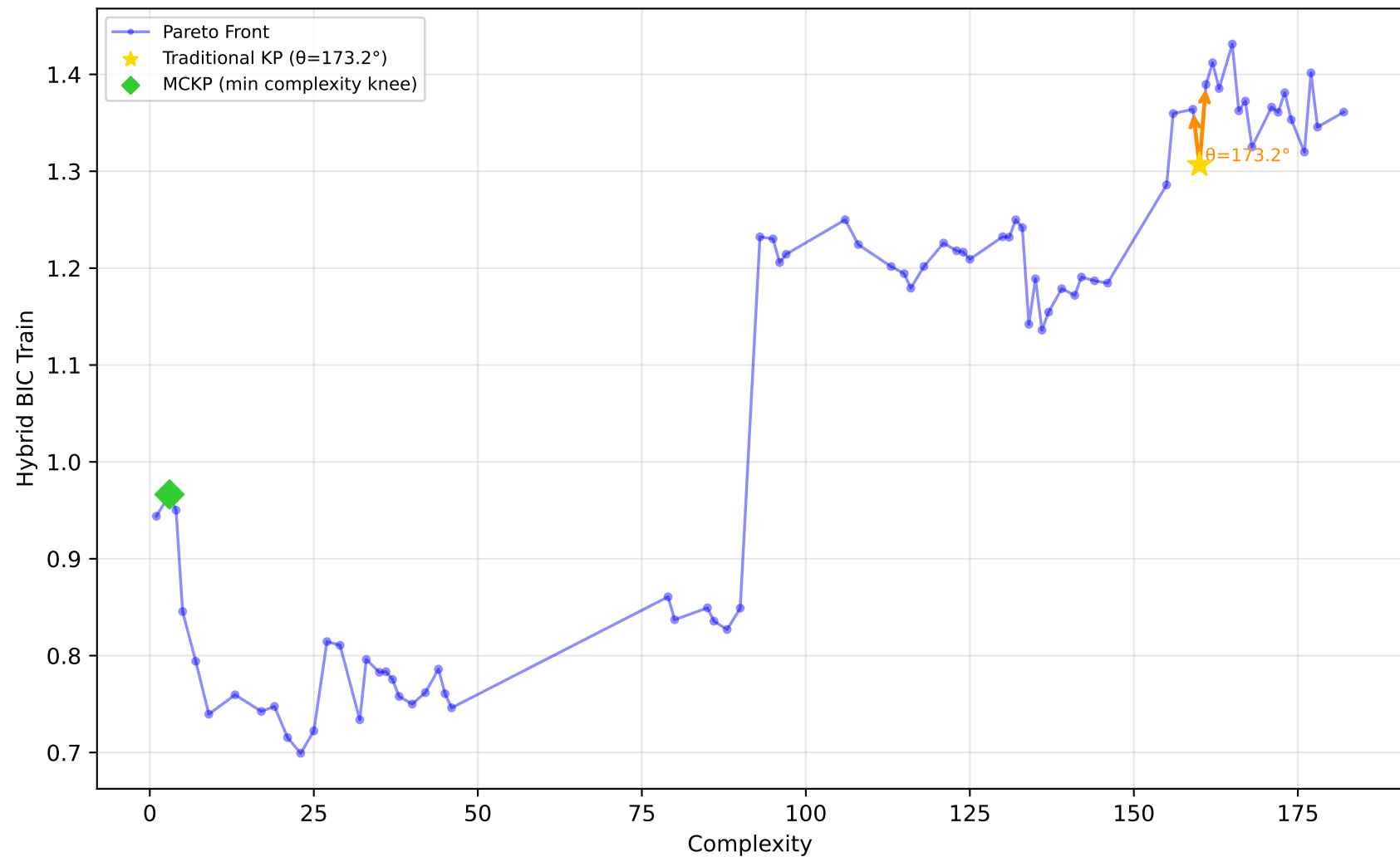
542_pollution - Run 30 - MVP - Hybrid BIC Train \lambda_1=0.40, \lambda_2=0.10, \lambda_3=0.00 | Difficulty: 0.24 | Method: mckp
