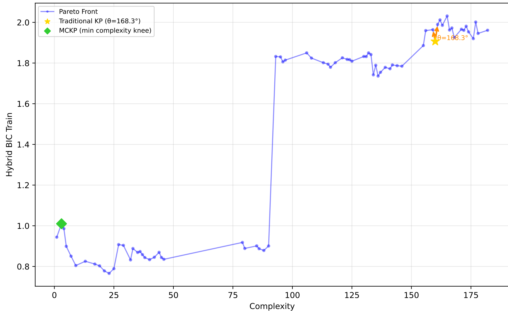
542_pollution - Run 30 - MVP - Hybrid BIC Train \lambda_1=1.00, \lambda_2=0.10, \lambda_3=0.00 | Difficulty: 0.24 | Method: mckp
