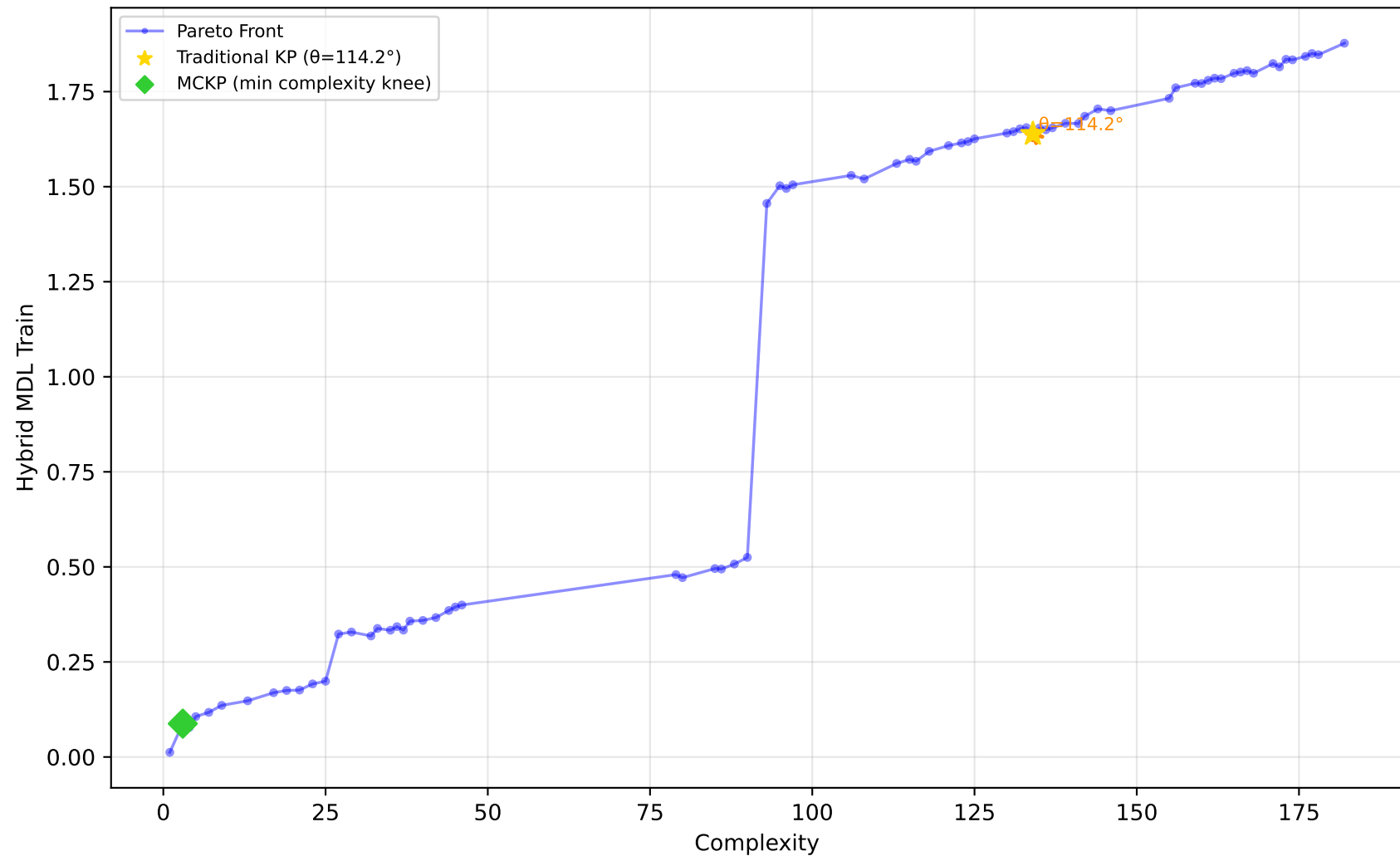
542_pollution - Run 30 - MVP - Hybrid MDL Train \lambda_1=1.00, \lambda_2=0.10, \lambda_3=0.00 | Difficulty: 0.24 | Method: mckp
