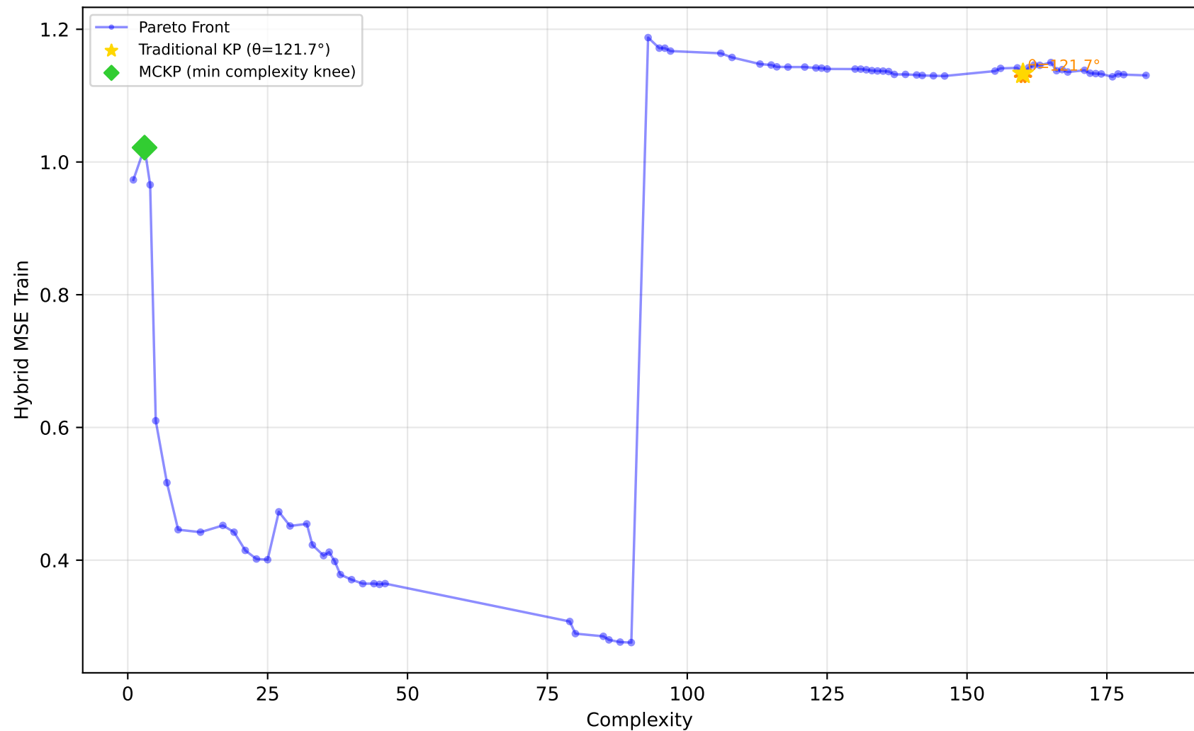
542_pollution - Run 30 - MVP - Hybrid MSE Train \lambda_1=1.00, \lambda_2=0.10, \lambda_3=0.00 | Difficulty: 0.24 | Method: mckp
