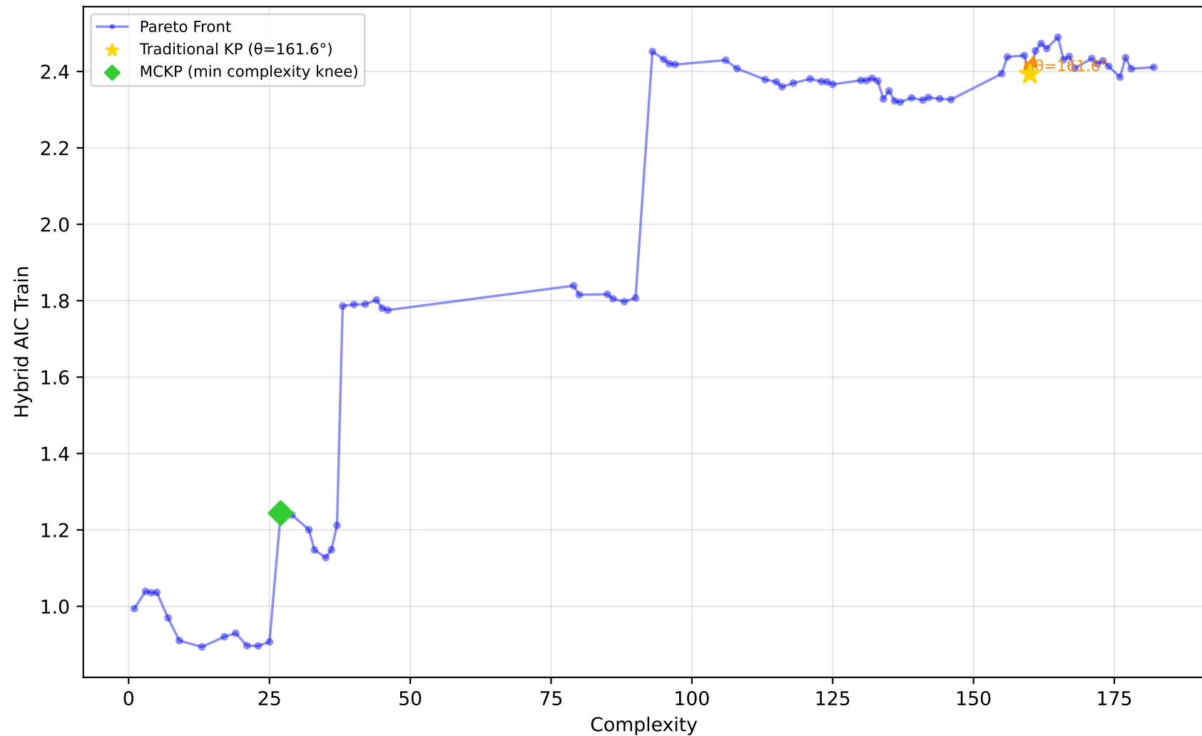
542_pollution - Run 30 - SVP - Hybrid AIC Train \lambda_1=0.70, \lambda_2=1.00, \lambda_3=0.10 | Difficulty: 0.24 | Method: mckp
