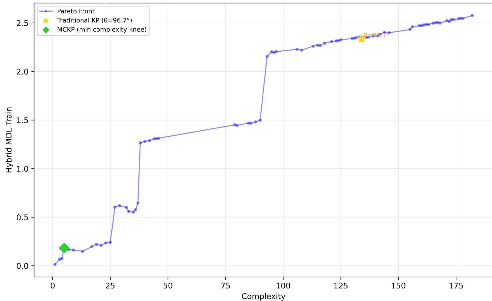
542_pollution - Run 30 - SVP - Hybrid MDL Train \lambda_1=0.70, \lambda_2=1.00, \lambda_3=0.10 | Difficulty: 0.24 | Method: mckp
