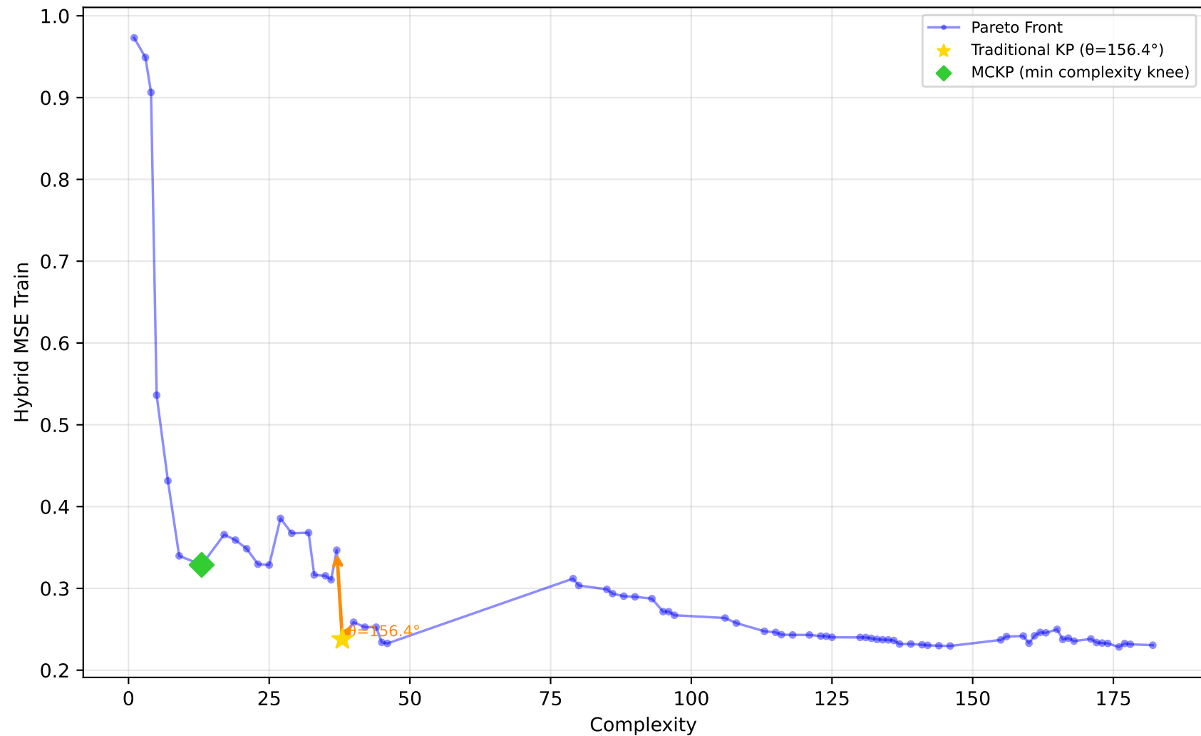
542_pollution - Run 30 - SVP - Hybrid MSE Train \lambda_1=0.00, \lambda_2=0.00, \lambda_3=0.20 | Difficulty: 0.24 | Method: mckp
