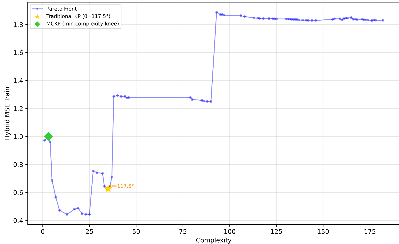
542_pollution - Run 30 - SVP - Hybrid MSE Train \lambda_1=0.70, \lambda_2=1.00, \lambda_3=0.10 | Difficulty: 0.24 | Method: mckp
