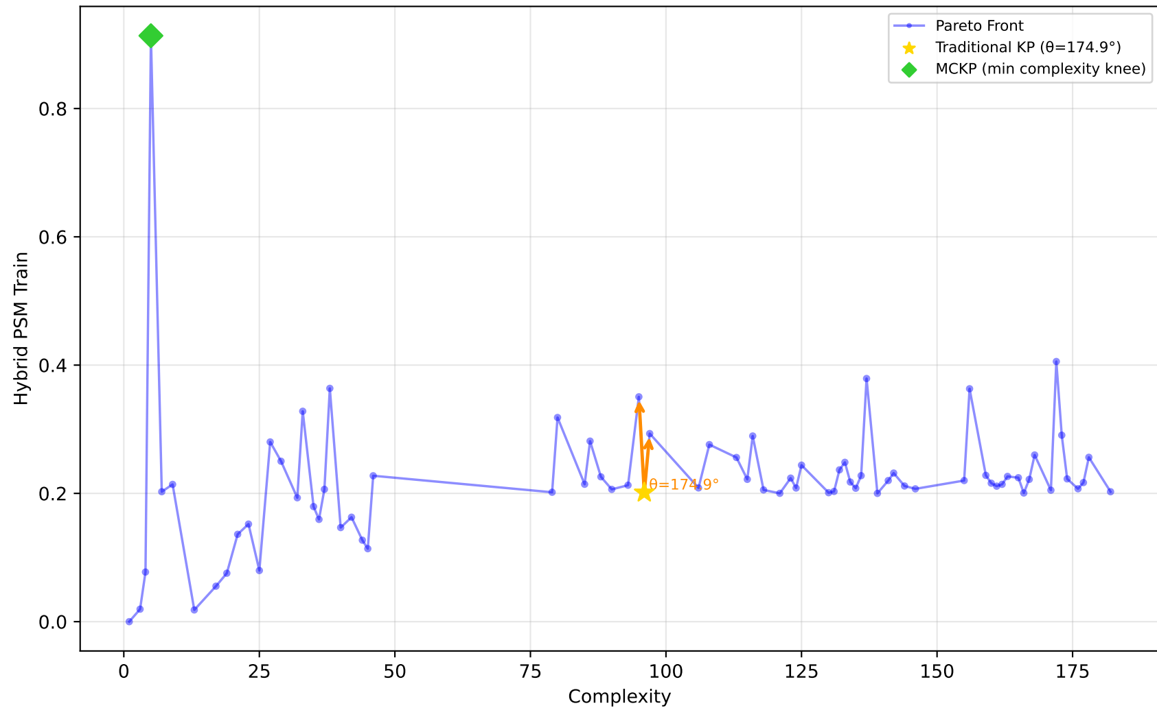
542_pollution - Run 30 - SVP - Hybrid PSM Train \lambda_1=0.00, \lambda_2=0.00, \lambda_3=0.20 | Difficulty: 0.24 | Method: mckp
