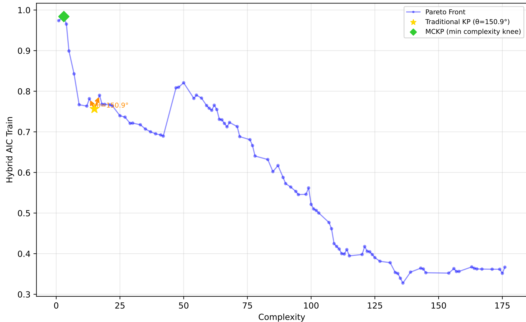
542_pollution - Run 3 - MVP - Hybrid AIC Train \lambda_1=0.40, \lambda_2=0.10, \lambda_3=0.00 | Difficulty: 0.30 | Method: mckp
