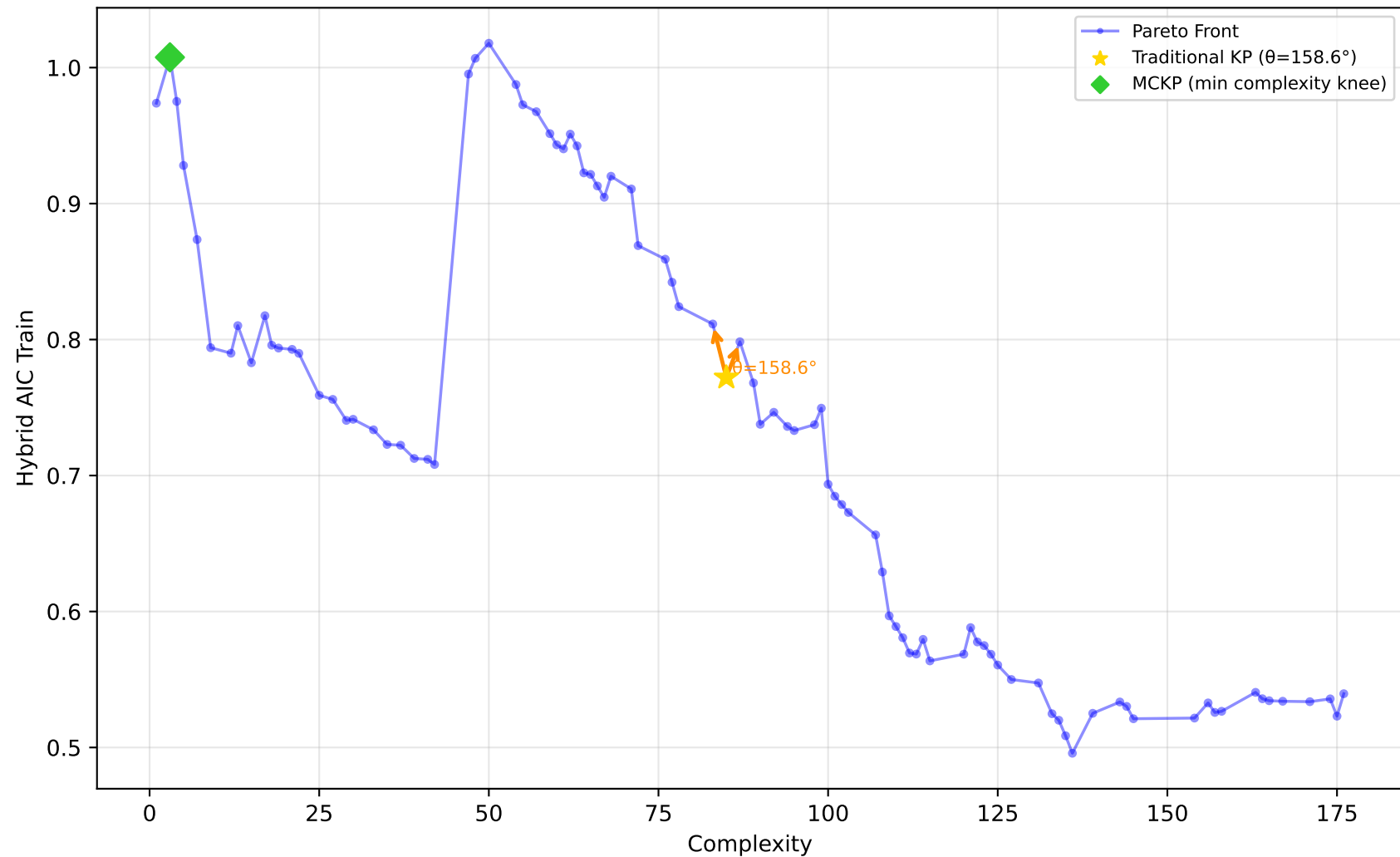
542_pollution - Run 3 - MVP - Hybrid AIC Train \lambda_1=1.00, \lambda_2=0.10, \lambda_3=0.00 | Difficulty: 0.30 | Method: mckp
