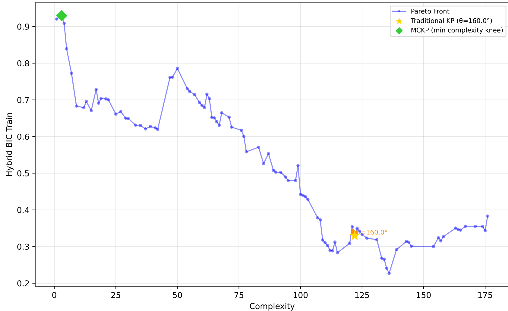
542_pollution - Run 3 - MVP - Hybrid BIC Train \lambda_1=0.40, \lambda_2=0.10, \lambda_3=0.00 | Difficulty: 0.30 | Method: mckp
