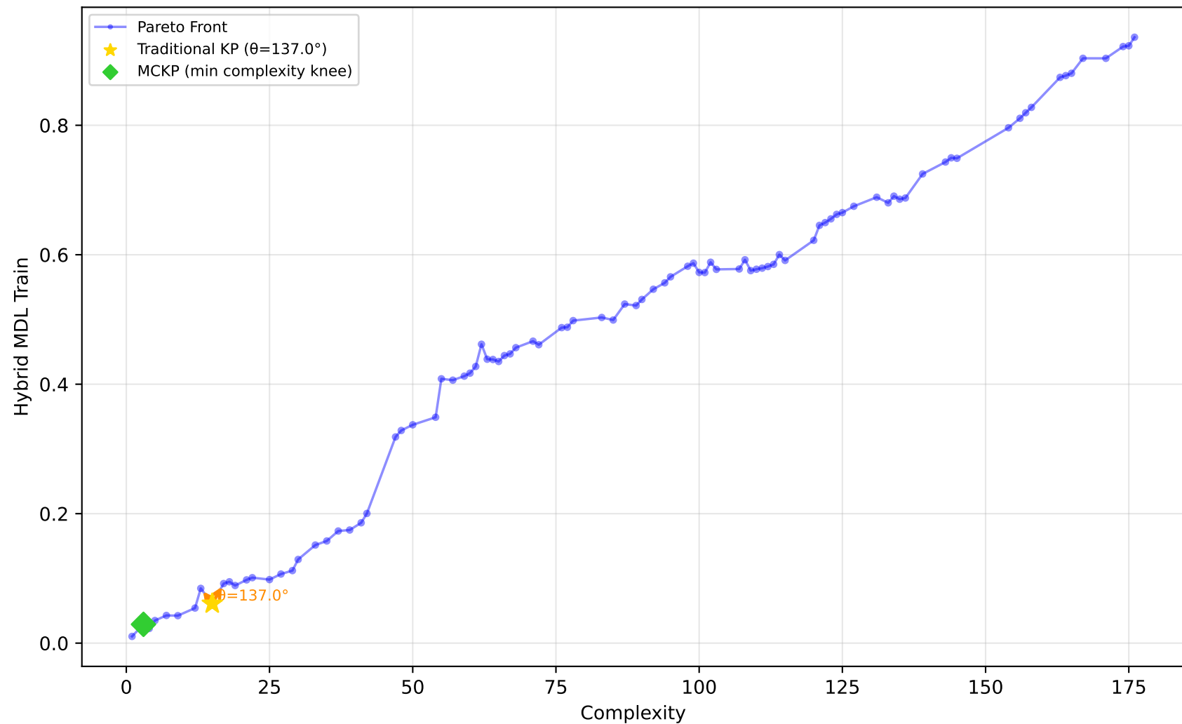
542_pollution - Run 3 - MVP - Hybrid MDL Train \lambda_1=0.40, \lambda_2=0.10, \lambda_3=0.00 | Difficulty: 0.30 | Method: mckp
