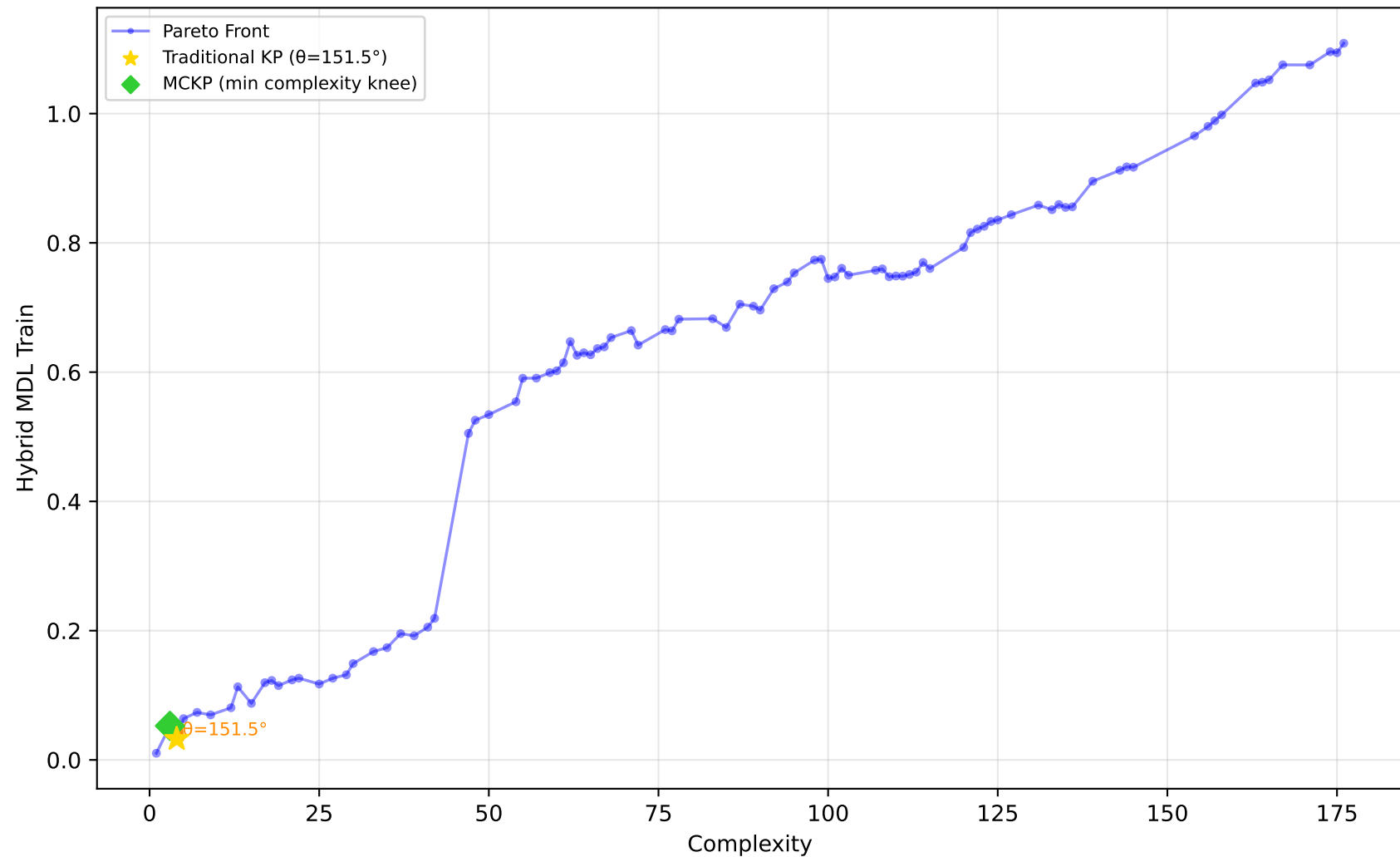
542_pollution - Run 3 - MVP - Hybrid MDL Train \lambda_1=1.00, \lambda_2=0.10, \lambda_3=0.00 | Difficulty: 0.30 | Method: mckp
