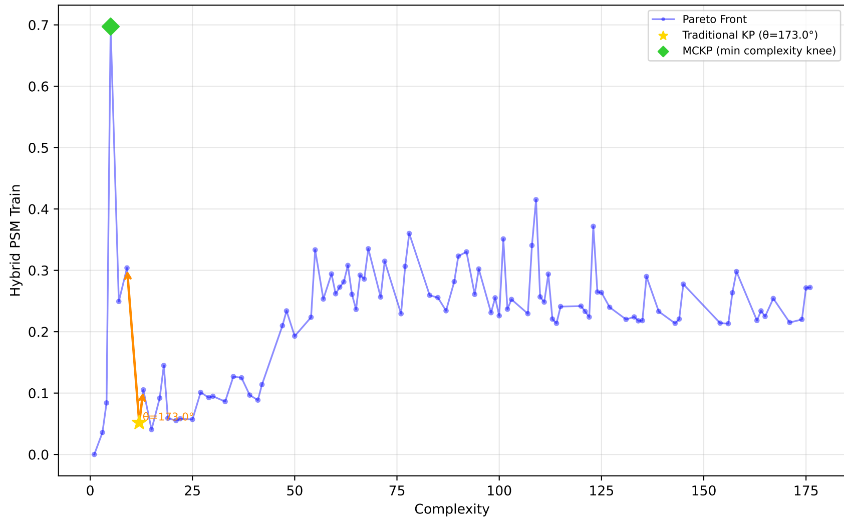
542_pollution - Run 3 - MVP - Hybrid PSM Train \lambda_1=0.40, \lambda_2=0.10, \lambda_3=0.00 | Difficulty: 0.30 | Method: mckp
