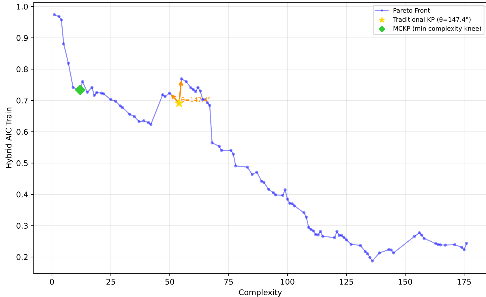
542_pollution - Run 3 - SVP - Hybrid AIC Train \lambda_1=0.00, \lambda_2=0.00, \lambda_3=0.20 | Difficulty: 0.30 | Method: mckp
