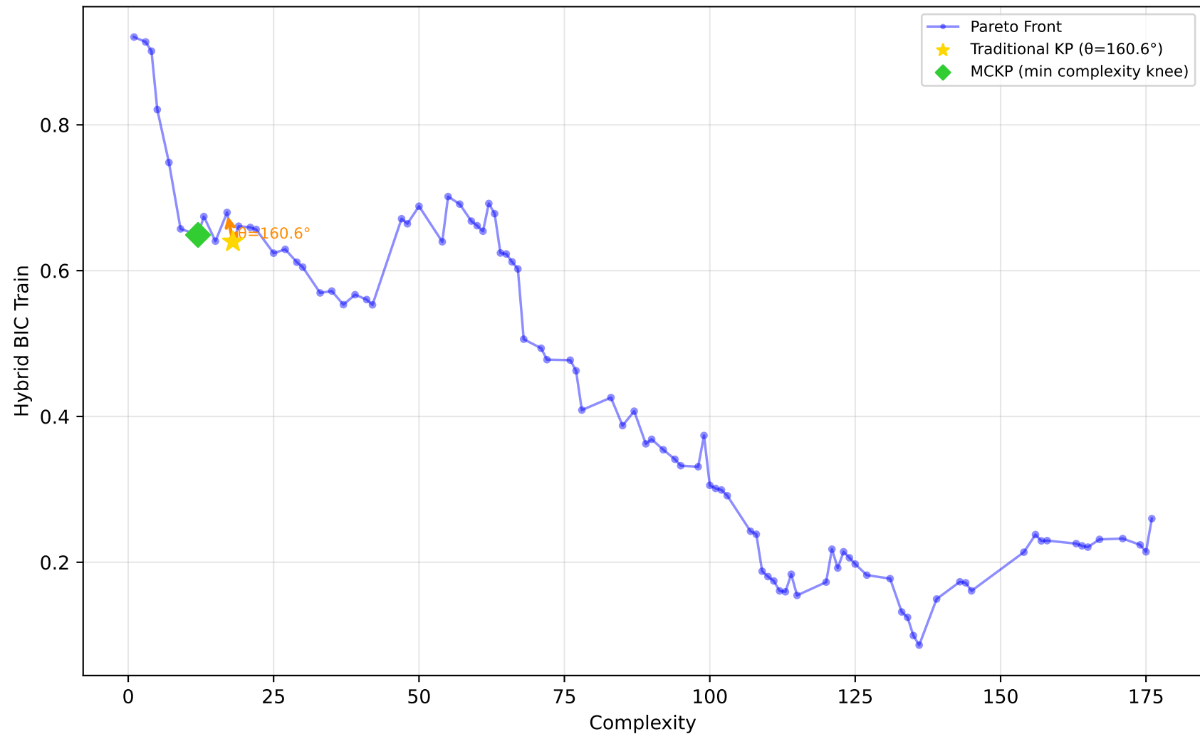
542_pollution - Run 3 - SVP - Hybrid BIC Train \lambda_1=0.00, \lambda_2=0.00, \lambda_3=0.20 | Difficulty: 0.30 | Method: mckp
