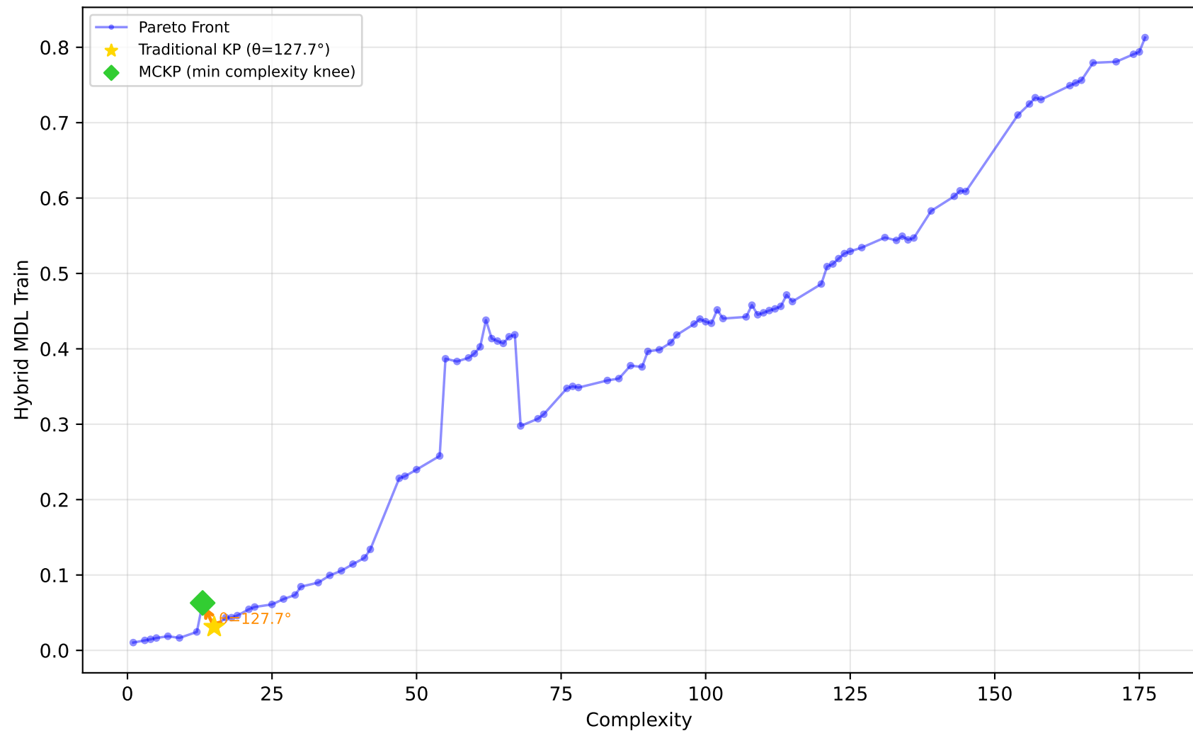
542_pollution - Run 3 - SVP - Hybrid MDL Train \lambda_1=0.00, \lambda_2=0.00, \lambda_3=0.20 | Difficulty: 0.30 | Method: mckp
