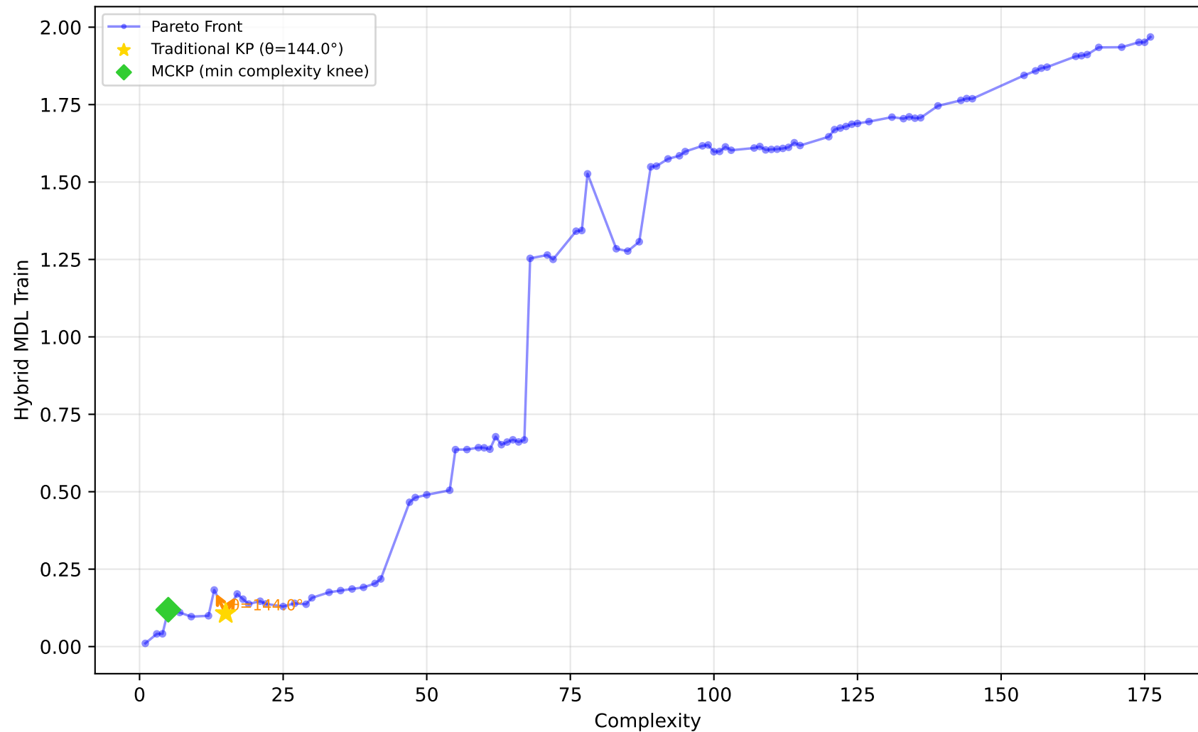
542_pollution - Run 3 - SVP - Hybrid MDL Train \lambda_1=0.70, \lambda_2=1.00, \lambda_3=0.10 | Difficulty: 0.30 | Method: mckp
