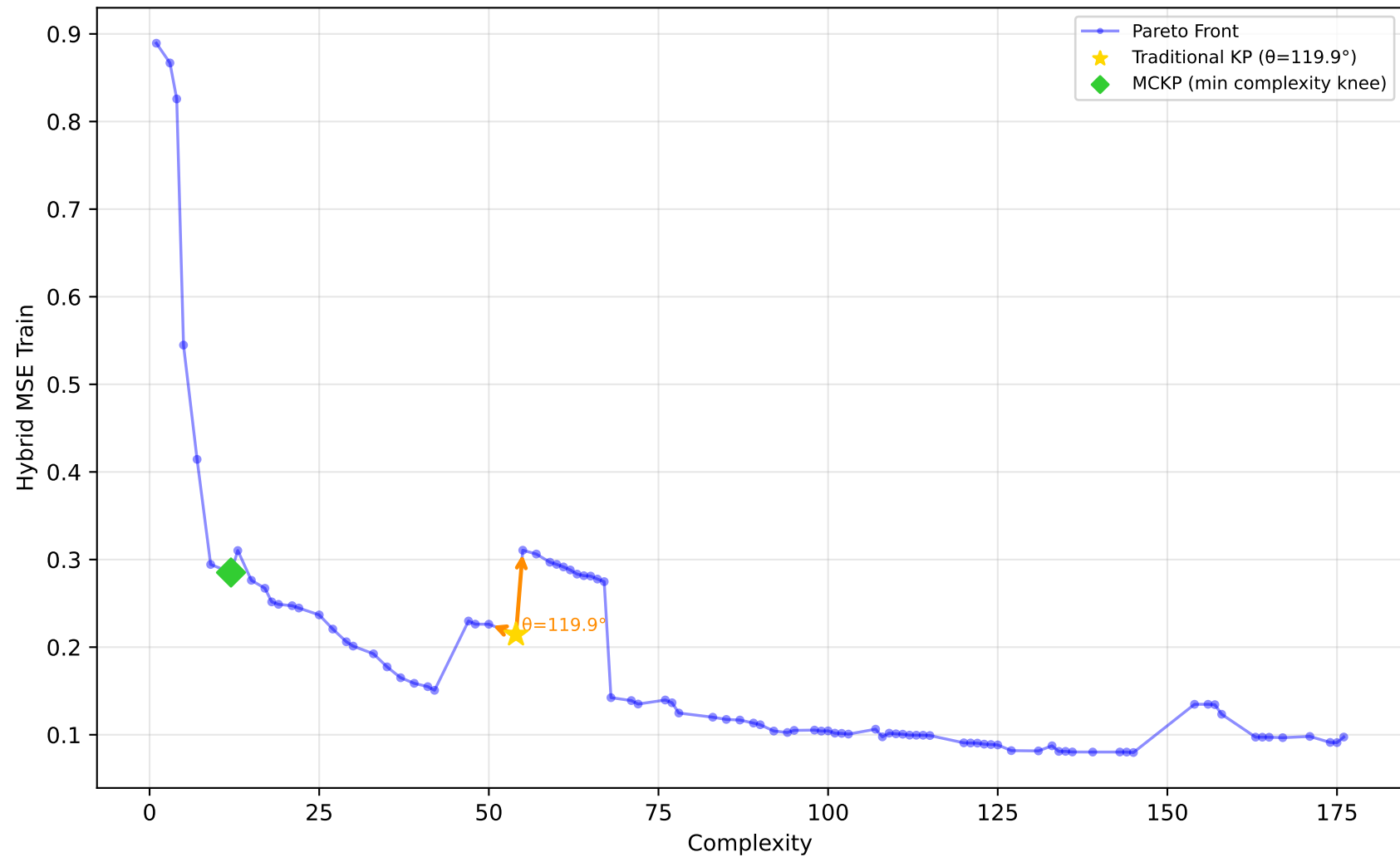
542_pollution - Run 3 - SVP - Hybrid MSE Train \lambda_1=0.00, \lambda_2=0.00, \lambda_3=0.20 | Difficulty: 0.30 | Method: mckp
