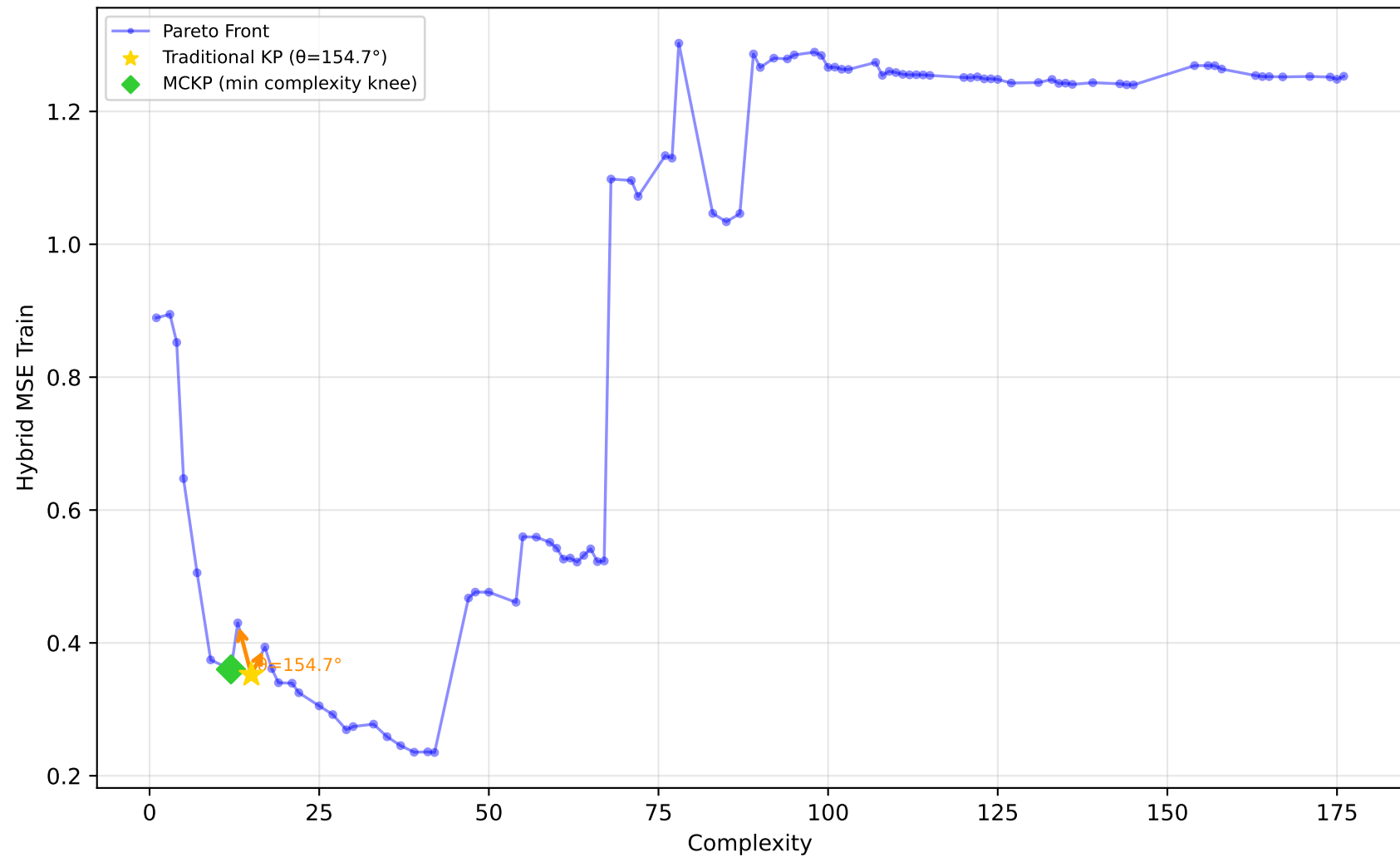
542_pollution - Run 3 - SVP - Hybrid MSE Train \lambda_1=0.70, \lambda_2=1.00, \lambda_3=0.10 | Difficulty: 0.30 | Method: mckp
