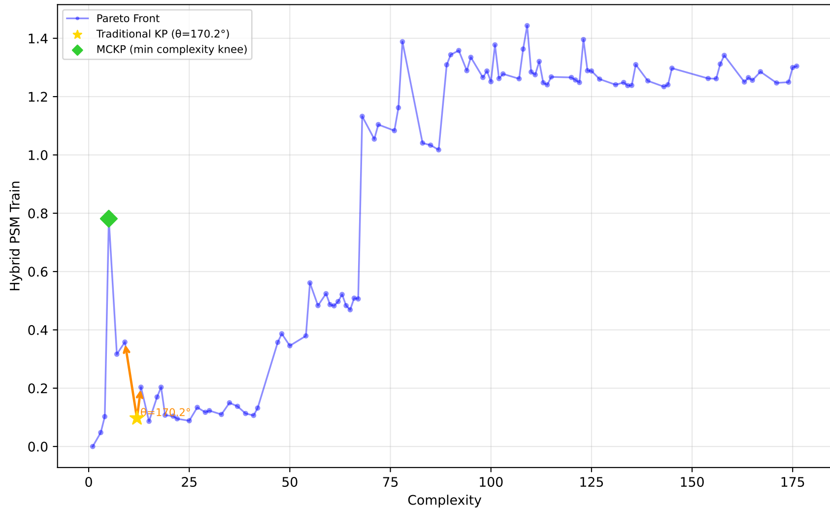
542_pollution - Run 3 - SVP - Hybrid PSM Train \lambda_1=0.70, \lambda_2=1.00, \lambda_3=0.10 | Difficulty: 0.30 | Method: mckp
