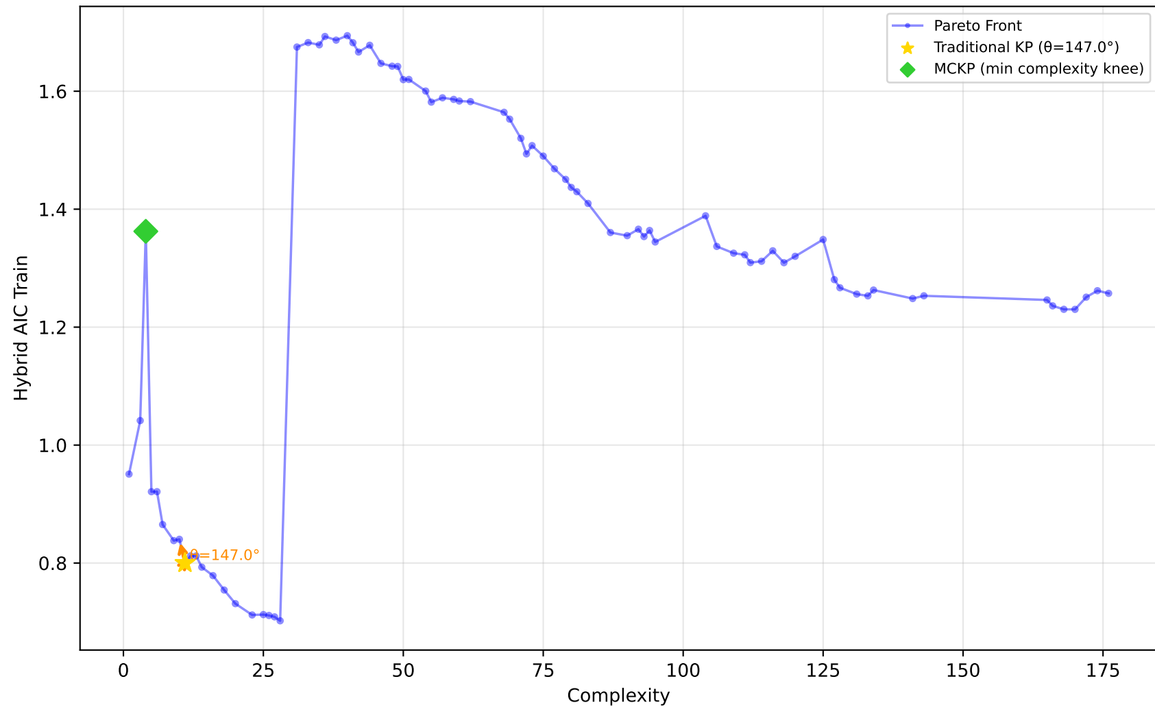
542_pollution - Run 4 - MVP - Hybrid AIC Train \lambda_1=1.00, \lambda_2=0.10, \lambda_3=0.00 | Difficulty: 0.48 | Method: mckp
