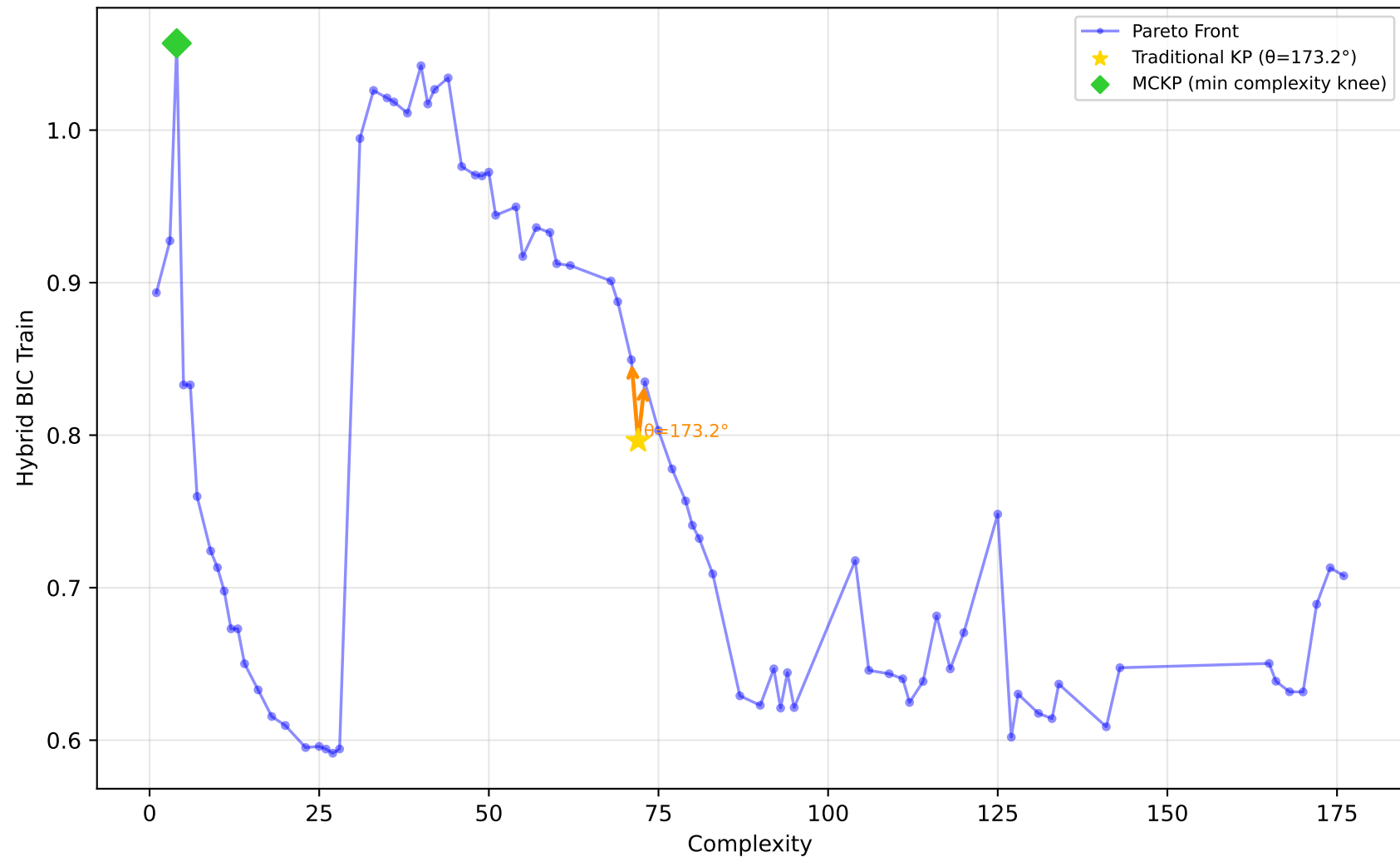
542_pollution - Run 4 - MVP - Hybrid BIC Train \lambda_1=0.40, \lambda_2=0.10, \lambda_3=0.00 | Difficulty: 0.48 | Method: mckp
