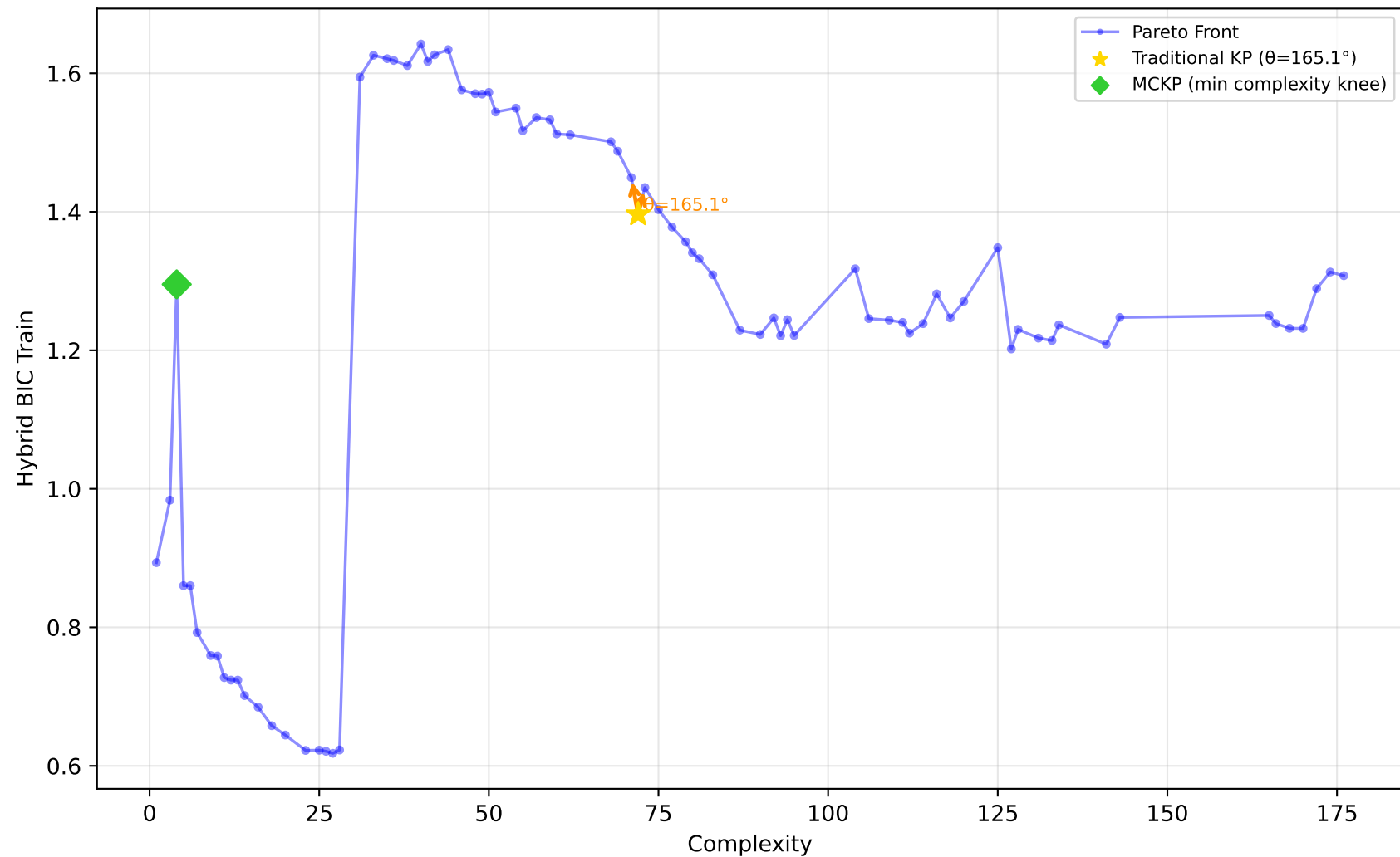
542_pollution - Run 4 - MVP - Hybrid BIC Train \lambda_1=1.00, \lambda_2=0.10, \lambda_3=0.00 | Difficulty: 0.48 | Method: mckp
