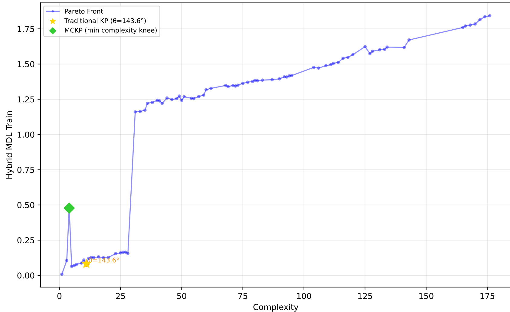
542_pollution - Run 4 - MVP - Hybrid MDL Train \lambda_1=1.00, \lambda_2=0.10, \lambda_3=0.00 | Difficulty: 0.48 | Method: mckp
