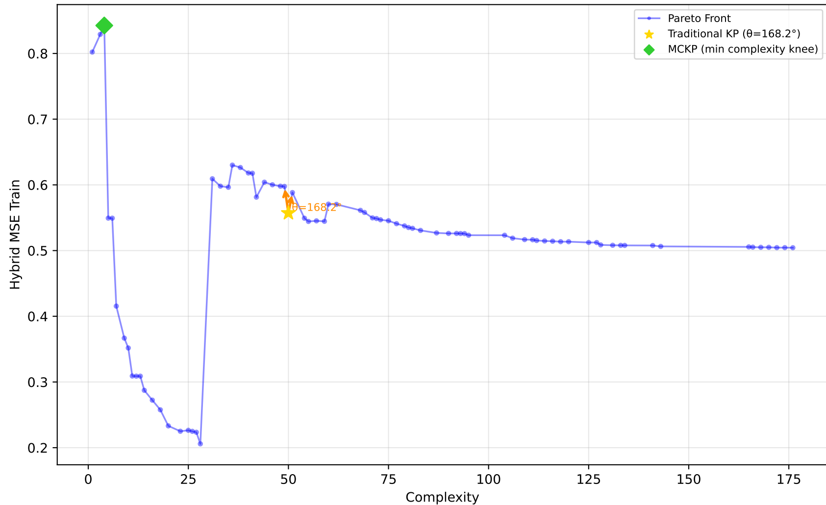
542_pollution - Run 4 - MVP - Hybrid MSE Train \lambda_1=0.40, \lambda_2=0.10, \lambda_3=0.00 | Difficulty: 0.48 | Method: mckp
