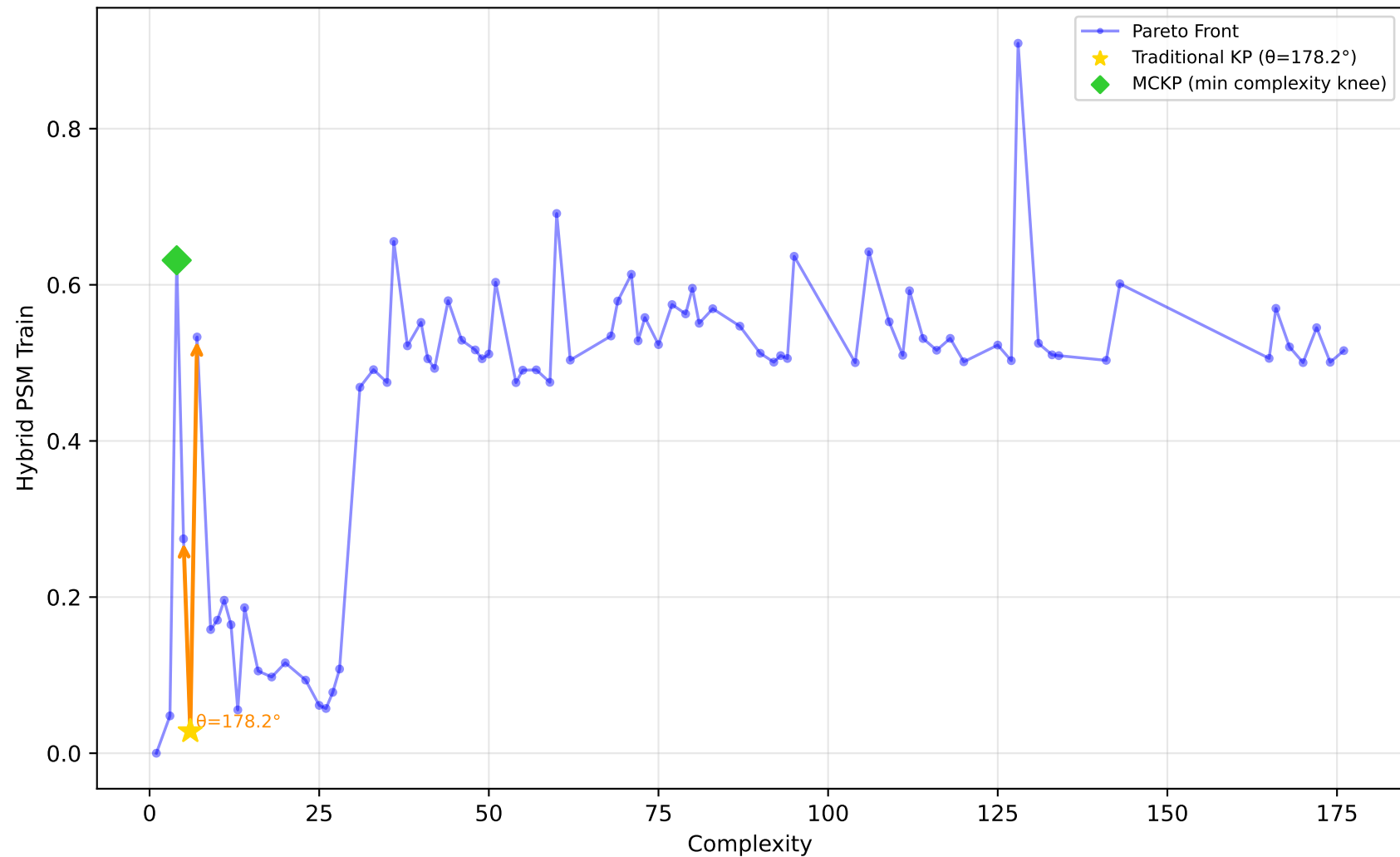
542_pollution - Run 4 - MVP - Hybrid PSM Train \lambda_1=0.40, \lambda_2=0.10, \lambda_3=0.00 | Difficulty: 0.48 | Method: mckp
