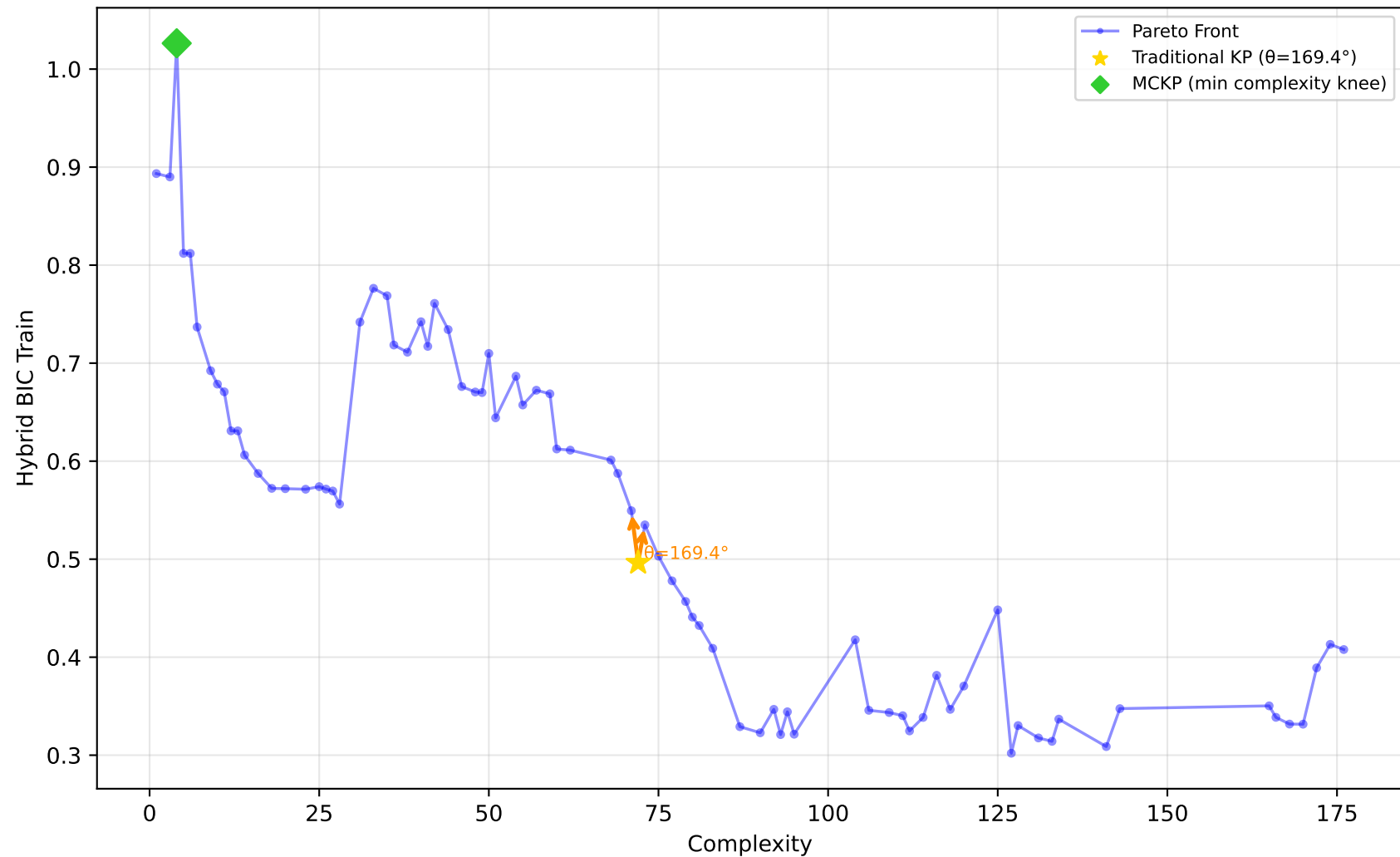
542_pollution - Run 4 - SVP - Hybrid BIC Train \lambda_1=0.00, \lambda_2=0.00, \lambda_3=0.20 | Difficulty: 0.48 | Method: mckp
