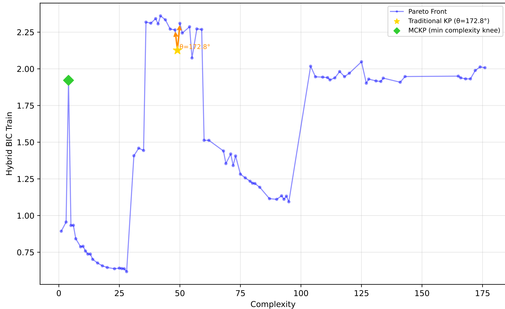
542_pollution - Run 4 - SVP - Hybrid BIC Train \lambda_1=0.70, \lambda_2=1.00, \lambda_3=0.10 | Difficulty: 0.48 | Method: mckp
