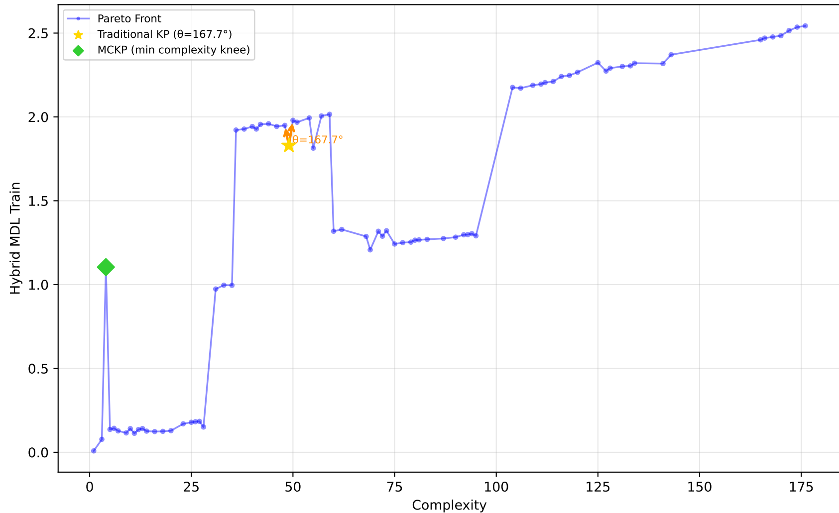
542_pollution - Run 4 - SVP - Hybrid MDL Train \lambda_1=0.70 , \lambda_2=1.00 , \lambda_3=0.10 | Difficulty: 0.48 | Method: mckp
