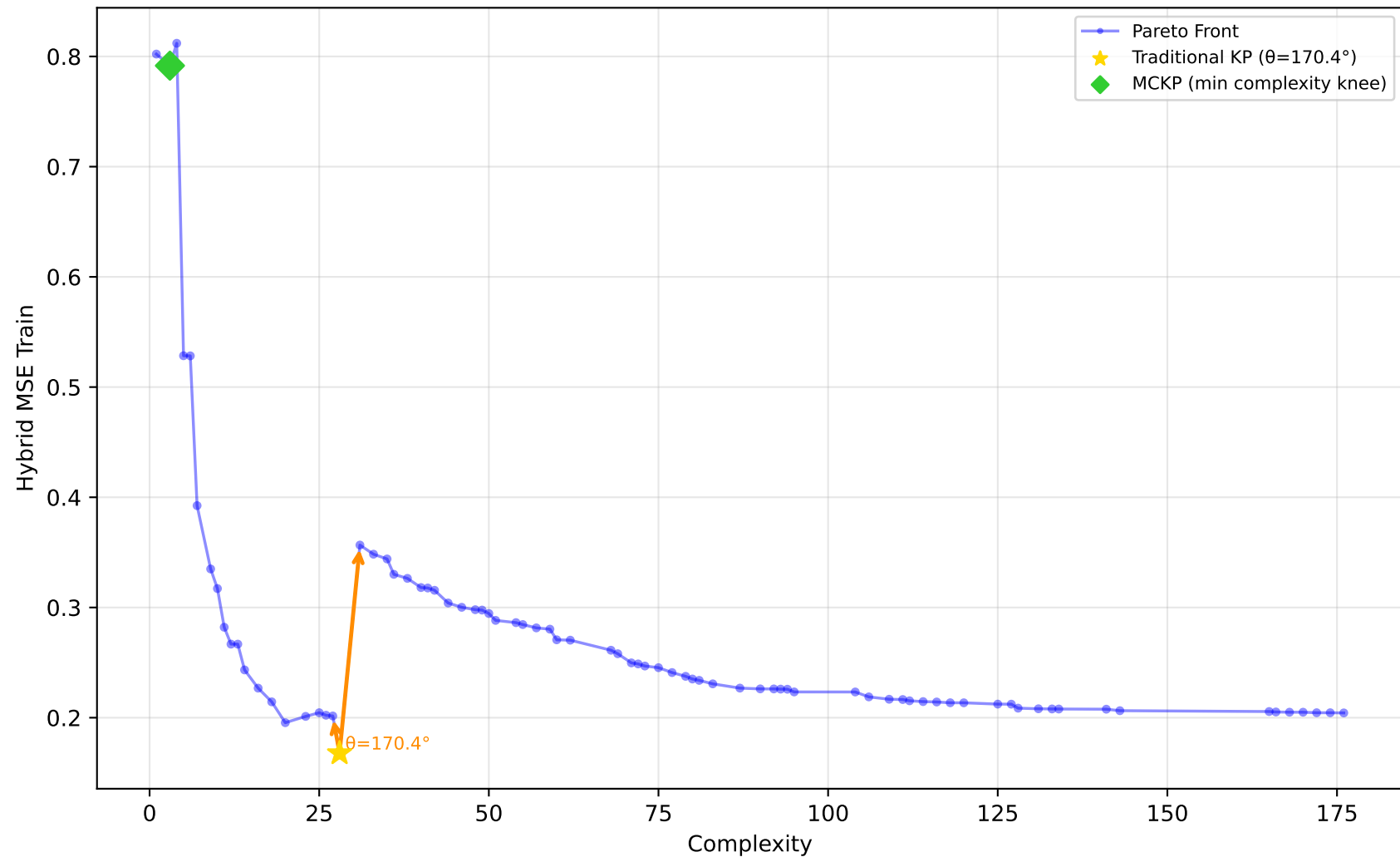
542_pollution - Run 4 - SVP - Hybrid MSE Train \lambda_1=0.00, \lambda_2=0.00, \lambda_3=0.20 | Difficulty: 0.48 | Method: mckp
