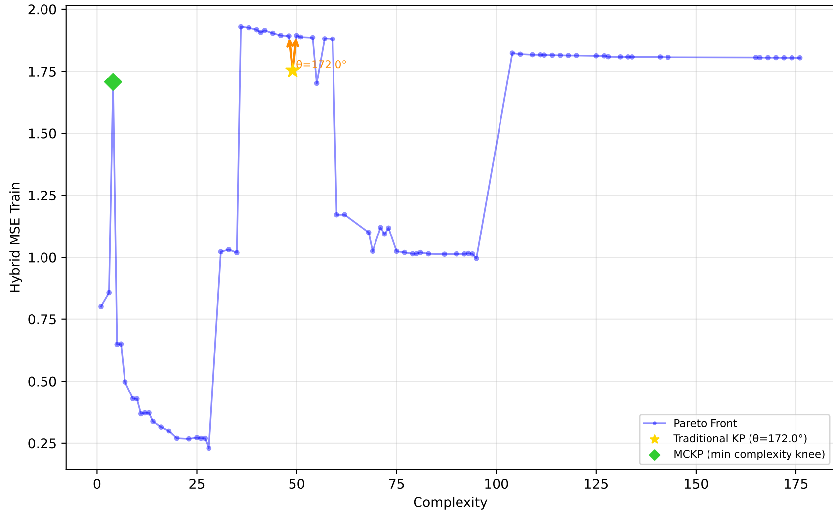
542_pollution - Run 4 - SVP - Hybrid MSE Train \lambda_1=0.70, \lambda_2=1.00, \lambda_3=0.10 | Difficulty: 0.48 | Method: mckp
