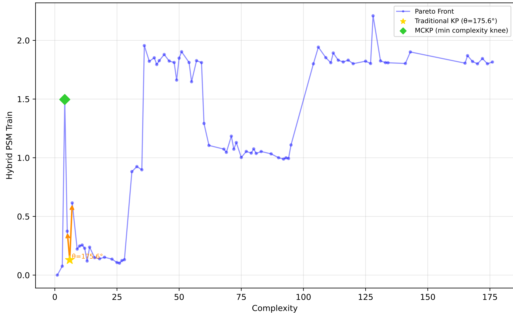
542_pollution - Run 4 - SVP - Hybrid PSM Train \lambda_1=0.70, \lambda_2=1.00, \lambda_3=0.10 | Difficulty: 0.48 | Method: mckp
