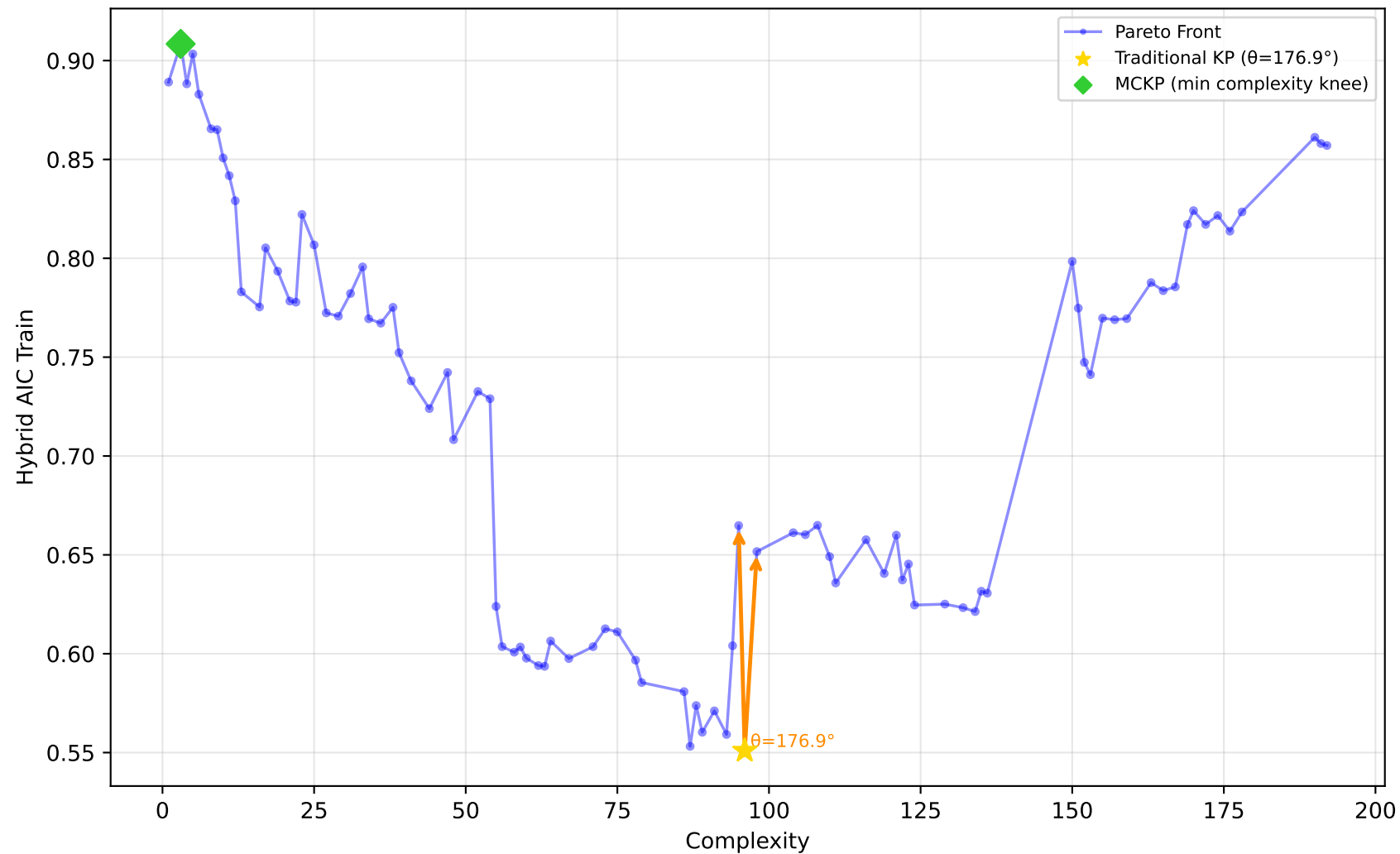
542_pollution - Run 5 - MVP - Hybrid AIC Train \lambda_1=0.40, \lambda_2=0.10, \lambda_3=0.00 | Difficulty: 0.59 | Method: mckp
