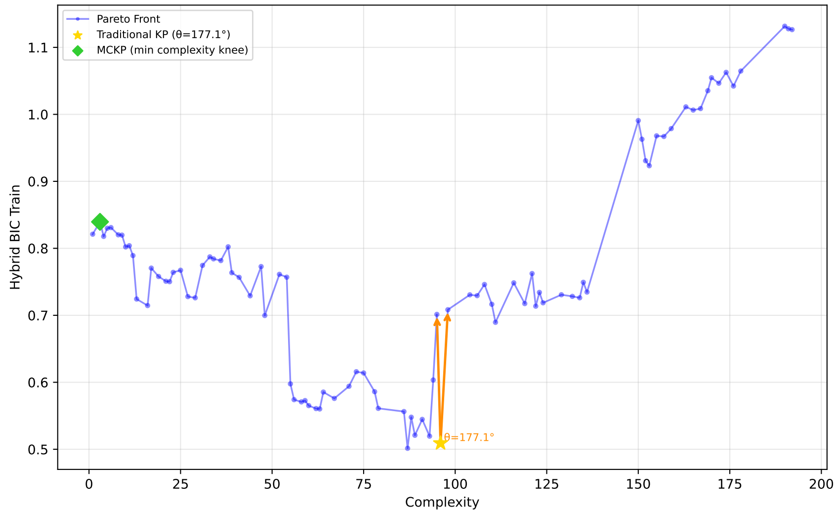
542_pollution - Run 5 - MVP - Hybrid BIC Train \lambda_1=0.40, \lambda_2=0.10, \lambda_3=0.00 | Difficulty: 0.59 | Method: mckp
