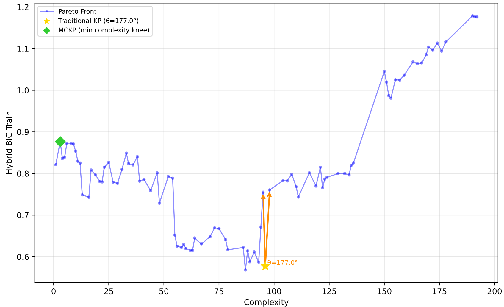
542_pollution - Run 5 - MVP - Hybrid BIC Train \lambda_1=1.00, \lambda_2=0.10, \lambda_3=0.00 | Difficulty: 0.59 | Method: mckp
